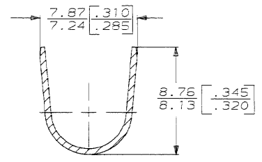
SECTION C-C SCALE 5:1
