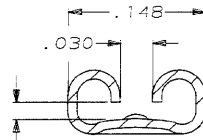
FITS .110 SERIES FASTON TABS SECTION A-A SCALE 10:1
