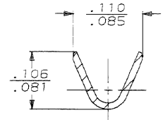
SECTION B-B SCALE 10:1
