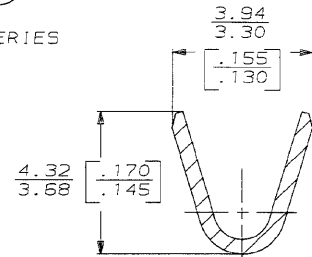
SECTION B-B SCALE 10:1
