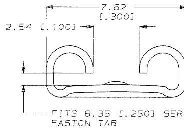
VIEW A-A SCALE 10:1
