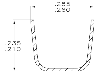
SECTION C-C SCALE 8:1
