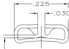
FITS .187 SERIES FASTON TAB VIEW A-A SCALE 8:1
