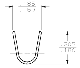
SECT. C-C
