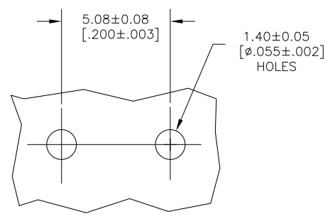
P.C. BOARD HOLE PATTERN
