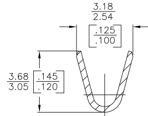
SECTION B-B SCALE 10:1
