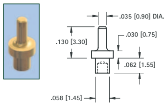
.035 (.90) PIN - SWAGE MOUNT
