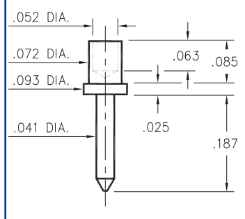
3145-2-00-XX-00-00-08-0 Swage mount in .076 hole. For .062 thick board
