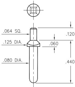
8952-0-05-XX-00-00-03-0 Square press-fit in .087 plated thru hole
