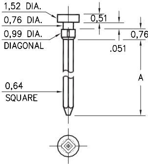
5275-X-05-XX-00-00-01-0 Square press-fit in 0,89 plated thru hole
