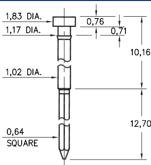
1215-3-05-XX-00-00-01-0 Press-fit in 1,09 mounting hole
