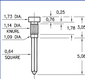
1124-0-05-XX-00-00-01-0 Press-fit in 1,09 mounting hole
