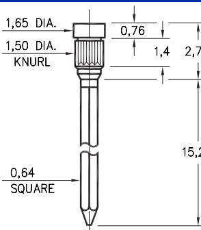
1094-0-05-XX-00-00-01-0 Press-fit in 1,42 mounting hole
