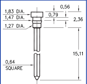
1222-0-05-XX-00-00-01-0 Press-fit in 1,40 mounting hole
