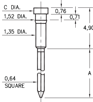
10XX-X-05-XX-00-00-01-0 Press-fit in 1,45 mounting hole
