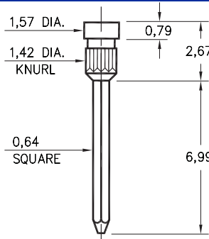
1210-0-05-XX-00-00-01-0 Press-fit in 1,35 mounting hole
