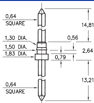
1221-0-05-XX-00-00-01-0 Press-fit in 1,42 mounting hole
