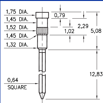
1110-3-05-XX-00-00-01-0 Press-fit in 1,45 mounting hole
