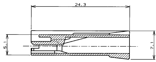
断面 "A-A" SECT.
