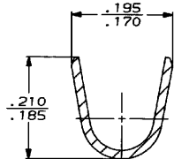
SECTION B-B SCALE 8:1
