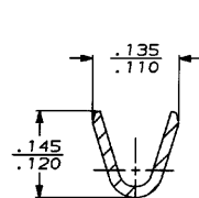
SECTION A-A SCALE 8:1
