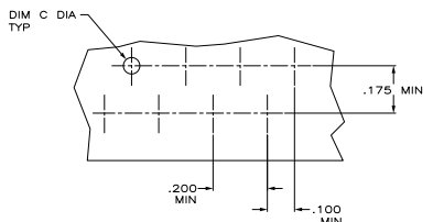
SUGGESTED PRINTED CIRCUIT BOARD MOUNTING DIMENSIONS
