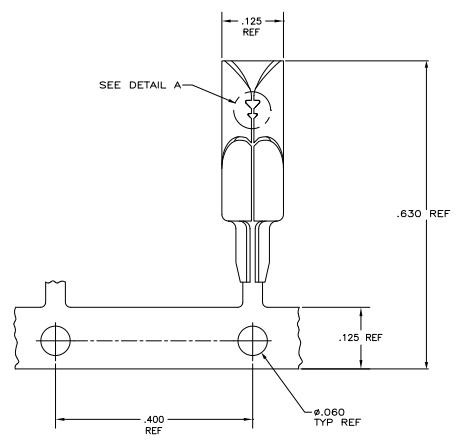
STRIP MOUNTED -2, -5 & -7 ONLY
