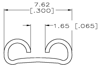
VIEW X-X SCALE 8:1
