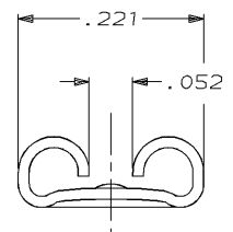
VIEW X-X SCALE 8:1
