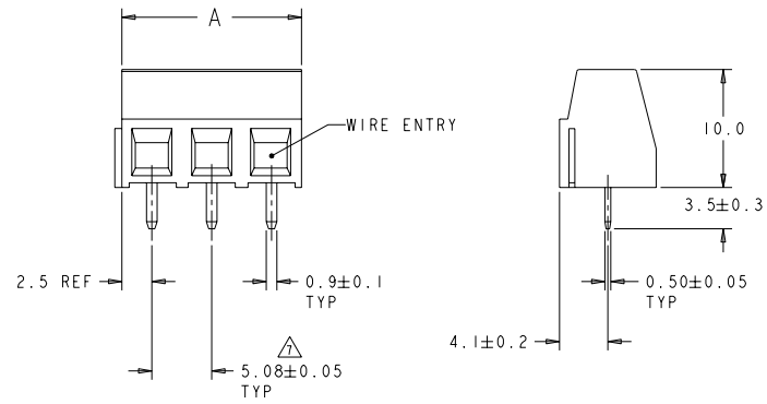
1546217-3 AS SHOWN
