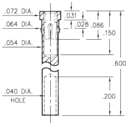
1707-0-19-XX-30-XX-10-0 Press-fit in .061 mounting hole
