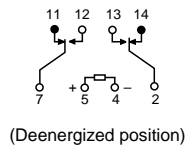
Schematic (Bottom view) Single side stable
