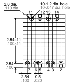
PC board pattern (Bottom view)
