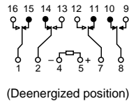
Schematic (Top view) Single side stable
