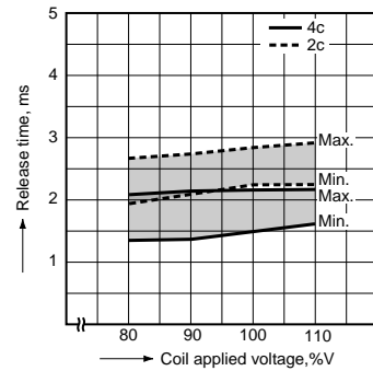
4. Release time (single side stable)
