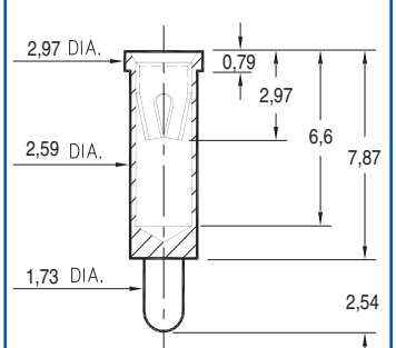
3044-0-15-XX-23-XX-04-0 Solder mount in 2,64 min. mounting hole
