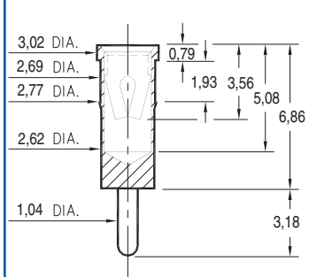
0492-0-15-XX-13-XX-04-0 Press-fit in 2,69 mounting hole
