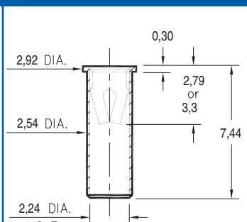
0362-0-15-XX-X3-XX-10-0 Solder mount in 2,59 min. mounting hole
