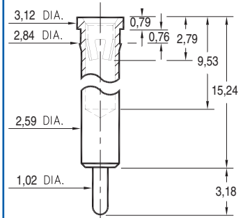
4034-0-15-XX-23-XX-04-0 Press-fit in 2,77 mounting hole
