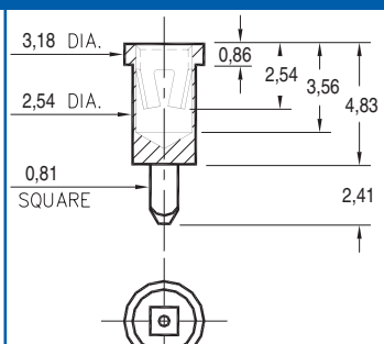
0367-0-15-XX-23-XX-10-0 Square press-fit in 1,02 plated thru hole
