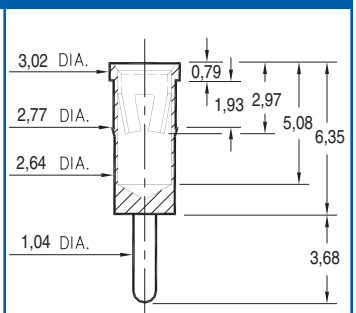
9324-0-15-XX-23-XX-04-0 Press-fit in 2,69 mounting hole
