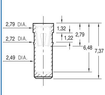
0381-0-15-XX-23-XX-10-0 Press-fit in 2,64 mounting hole
