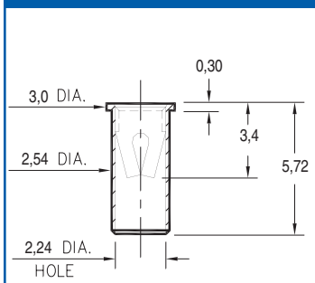
0372-0-15-XX-13-XX-10-0 Solder mount in 2,59 min. mounting hole
