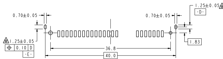
ALTERNATIVE P.C.B. LAYOUT REFER TO RECOMMENDED PCB LAYOUT FOR UNSPECIFIED DIMENSIONS TOLERANCE UNLESS OTHERWISE \pm 0.10
