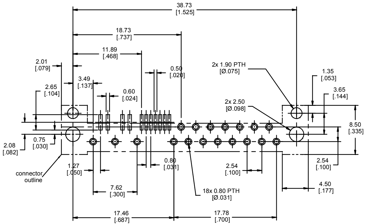
RECOMMENDED PCB LAYOUT (PCB=2.36mm)
