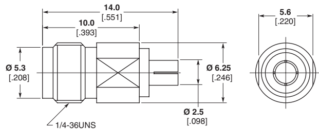
Part Number 1775230-1
