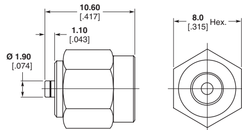
Part Number 1775227-1
