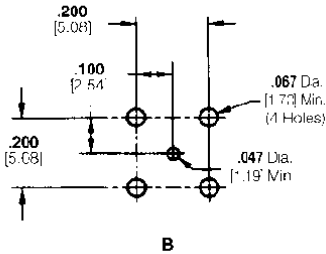
Recommended PC Board Layouts
