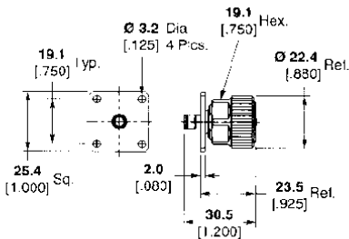
Part No. 1061750-1 M/A-COM Model No. 7082-2242-00
