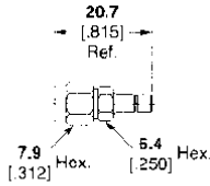
Part No. 1060500-1 M/A-COM Model No. 5182-2241-00
