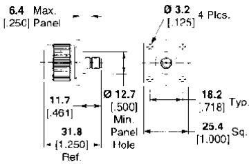
Part No. 1057383-1 M/A-COM Model No. 3082-2242-00
