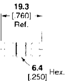
Part No. 1060498-1 M/A-COM Model No. 5182-2240-00
