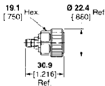
Part No. 1053788-1 M/A-COM Model No. 2082-2700-00
