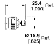
Part No. 1057853-1 M/A-COM Model No. 3182-2240-00
