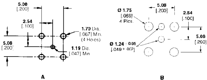
Recommended PC Board Layouts
