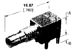
Bulkhead Jack
