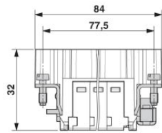
Male insert
