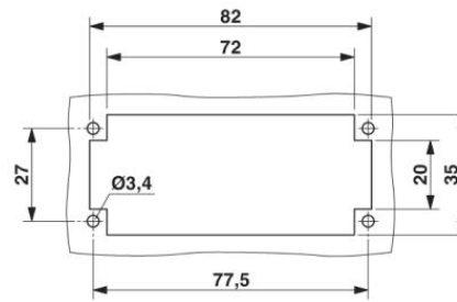
Mounting cut-out
