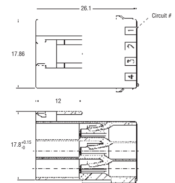
Section X-X
