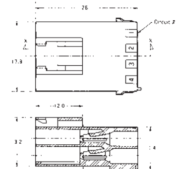
Section X-X
