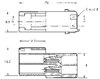
Section X-X
