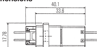
Panel/Free-Hanging Type
