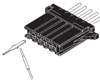
② Extract contacts from Board-mounting Vertical Type connector and insert them for testing.
