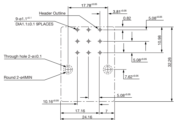
PC Board Layout Applicable Board Thickness: 1.6±0.1
