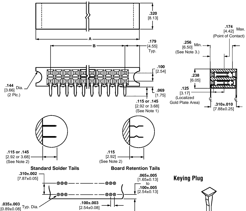
Standard Solder Tails Board Retention Tails Recommended PC Board Hole Layout (for .055 [1.40] min. thick PC board)
