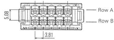
Horizontal/Vertical Type
