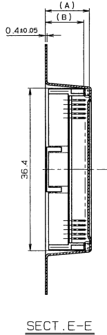
SECT. E-E
