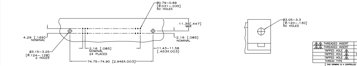
DETAIL C (THRU-BOLT)
