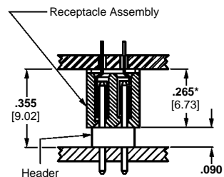
Figure 2 Double-Row, Mod IV, Top Entry, Breakaway Header
