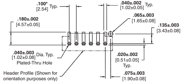
Recommended PC Board Hole Layout (Stencil Thickness = .010 [0.25])
