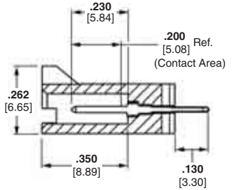
Section X-X
