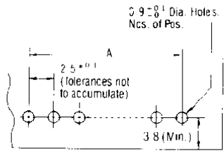
PC Board Layout (Applicable board thickness: 1.6mm)
