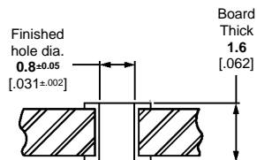
Solder Post
