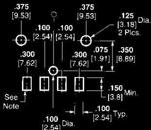
Note: .010 [.25] min. thick solder paste, 63/27 Recommended PC Board Layout .062 [1.57] thick PC Board
