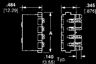
Part Number 770829-1
