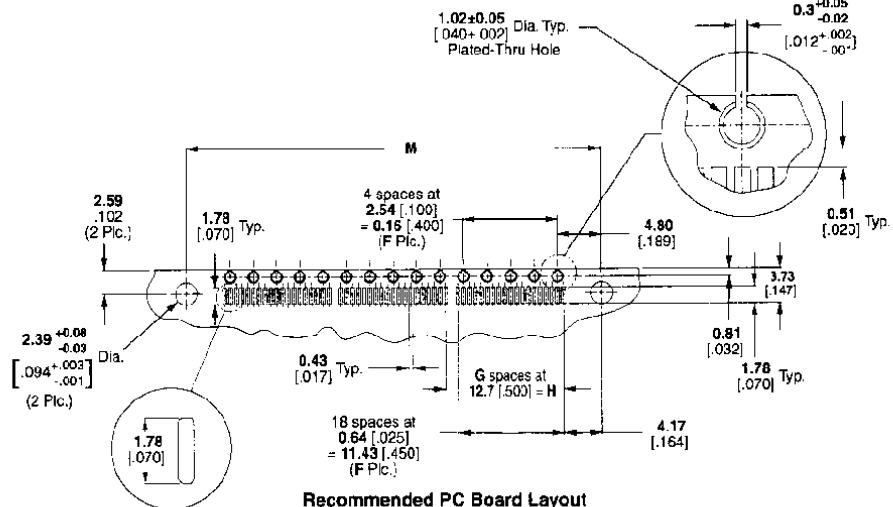
Recommended PC Board Layout (Mirror image on opposite side) PC Board Thickness: 1.57 [0.062]
