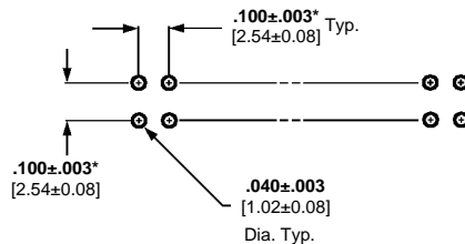
Recommended PCBoard Hole Layout For Manual Insertion
