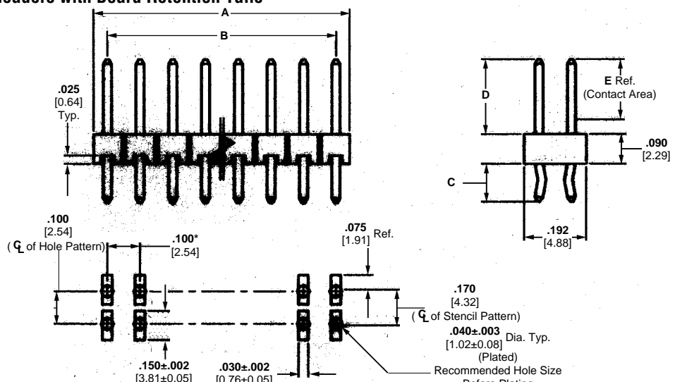
Recommended PC Board Mounting Pattern (for .062 [1.57] thick PC board; .008 [2.03] thick stencil)
