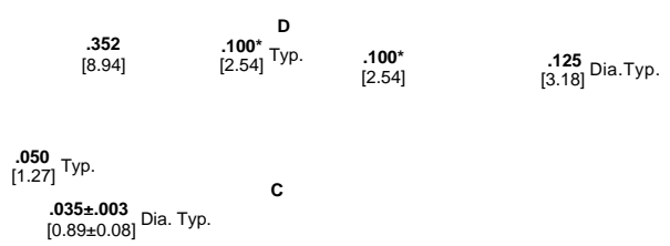
Recommended PC Board Hole Layout (for .055 [1.40] min. thick PC board)
