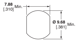
Suggested Panel Cutout
