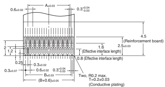
Applicable FPC Dimensions
