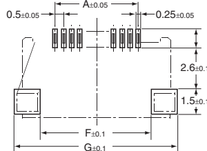
PCB Mating Dimensions (Top View)
