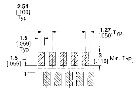
Surface Mount Recommended PC Board Layout
