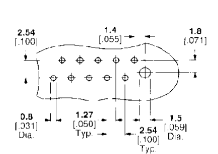
Through Hole Recommended PC Board Layout
