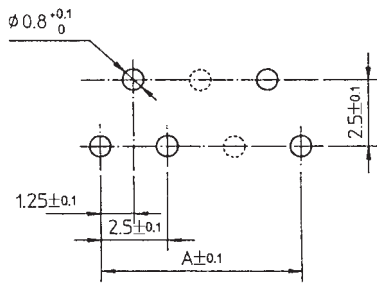
基板穴寸法 (コネクタ群縦断面) MOUNTING LAYOUT (適用基板厚 t=1~1.6) (t=1~1.6)
