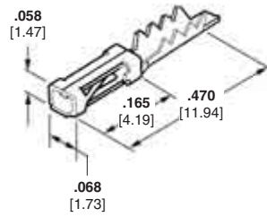
No-Strip Receptacle
