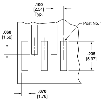
Recommended PC Board Layout for use with .010 [0.25] Thick Stencil
