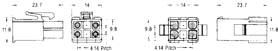
Plug
