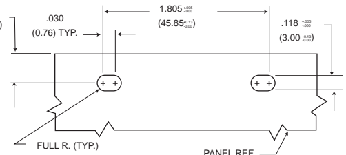
Figure 3 Edgeboard Mounting
