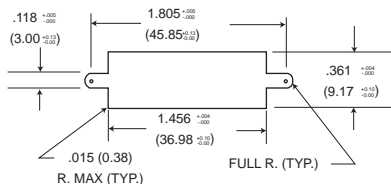
Figure 1 Front Mounting
